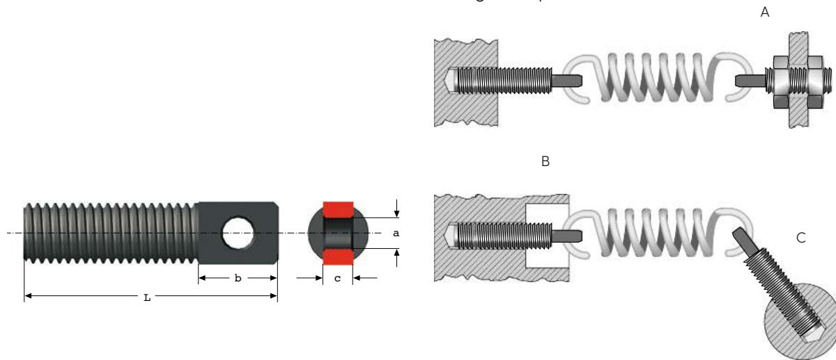
Fitting example
