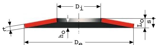
Group 1 and Group 2 springs
