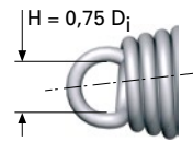
11. Coned spring with reduced loop
